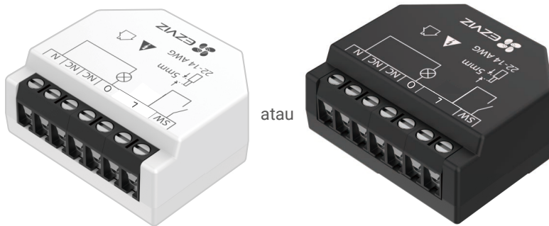
Relai Wi-Fi (×1)
